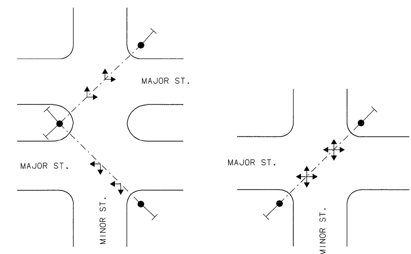
TYPICAL SPAN WIRE INSTALLATIONS
