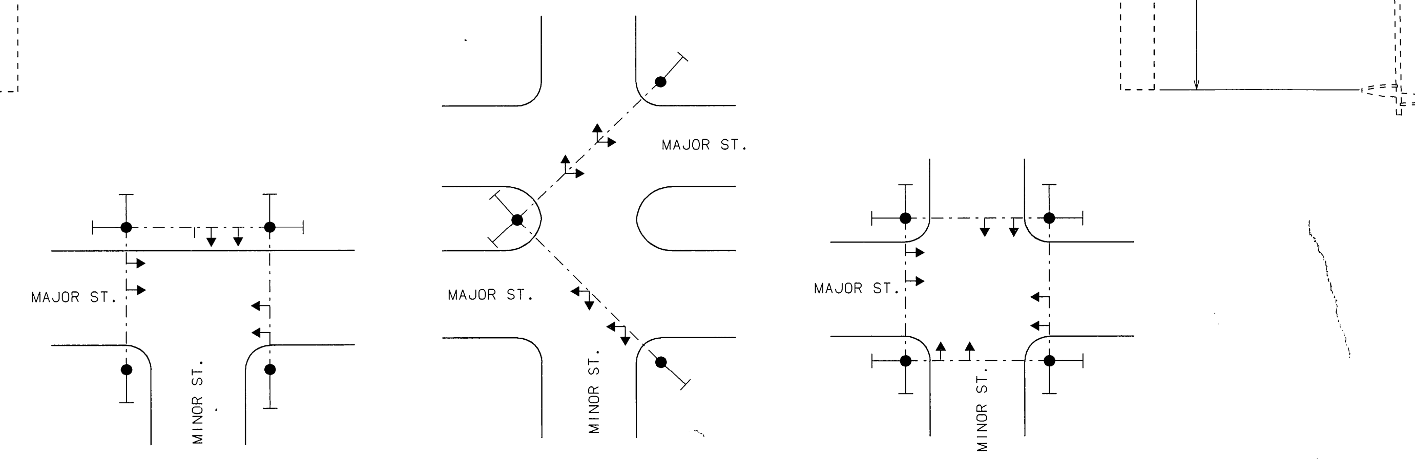
TYPICAL SPAN WIRE INSTALLATIONS
