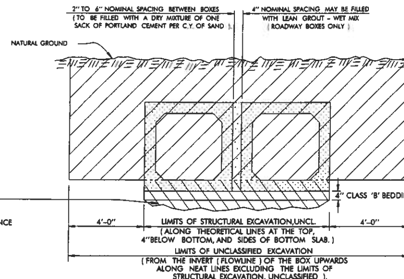
REQUIREMENTS FOR EXCAVATION OF PRECAST R.C.B. STORM SEWERS
