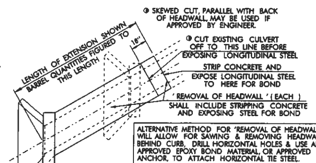
ALTERNATE METHOD FOR EXTENDING NON-0° SKEWED BOXES
