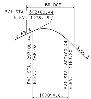
PROFILE GRADE - RAMP 44A
