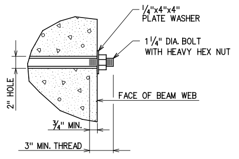
DIAPHRAGM BOLT DETAIL
