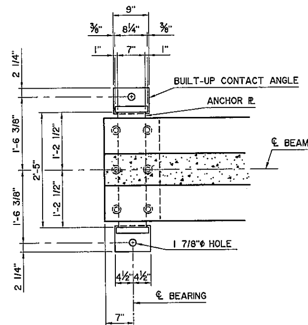
FIXED BEARING PLAN
