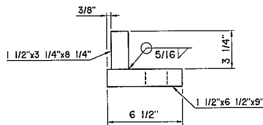
BUILT-UP CONTACT ANGLE DETAIL
