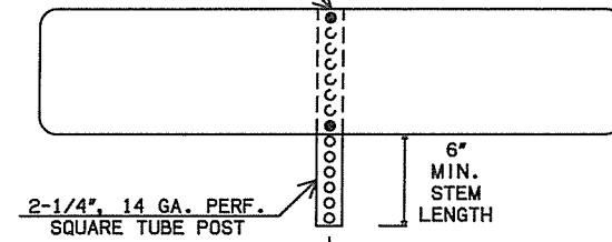
SIGN 13 INSERT DETAIL NOT TO SCALE
