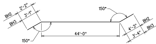
BH2 - #4 BAR x 50'-5"
