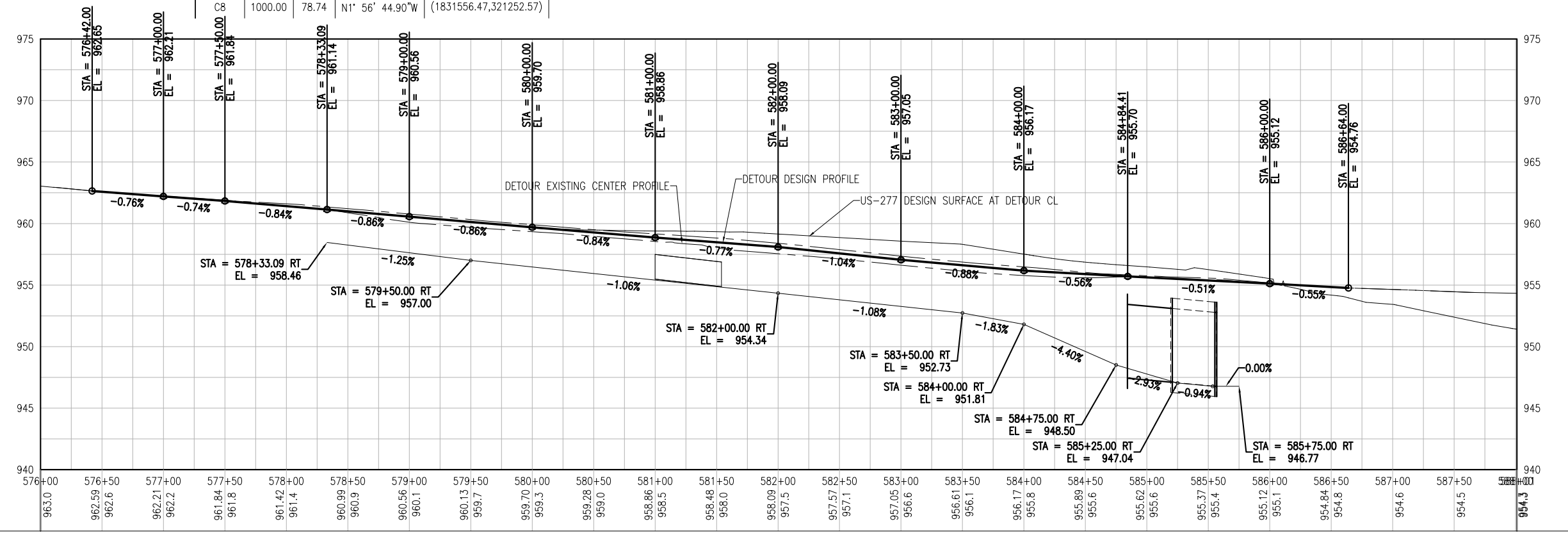
Alignment - DETOUR PH 1 SOUTH PROFILE
