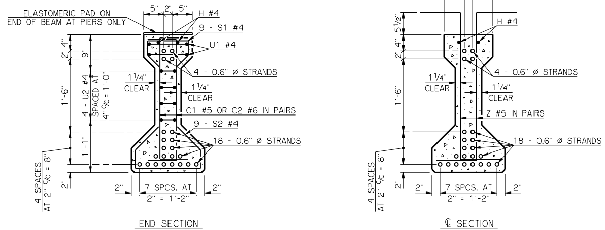
END SECTION
