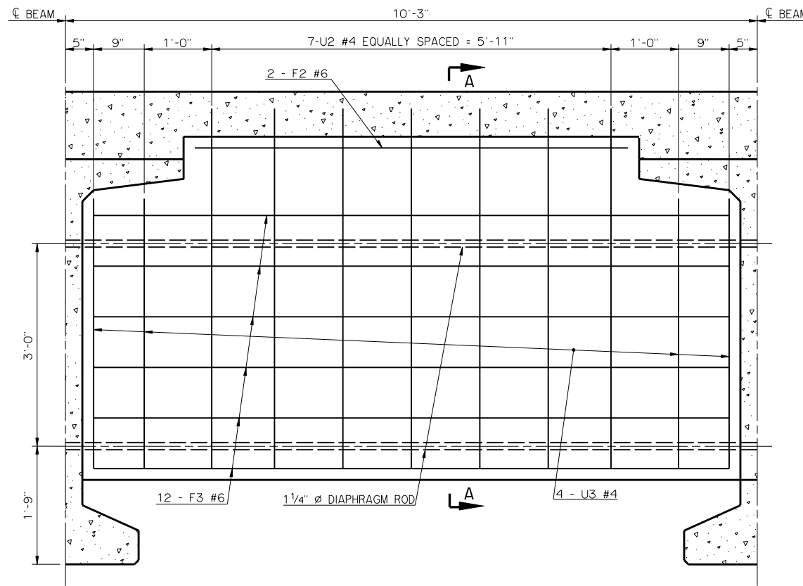
ELEVATION OF END DIAPHRAGM
